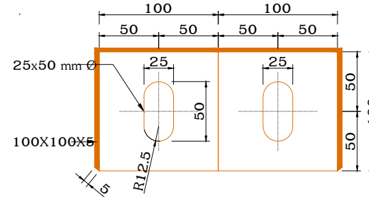
DOUBLE BACKUP PLATE
