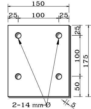
GIRT CLIP
