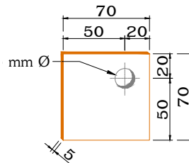
GUSSET PLATE
