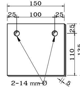
END GIRT CLIP-01
