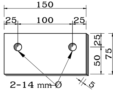
END GIRT CLIP
